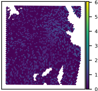
SNU51A EFNB3 expression Moran's I = 0.07
