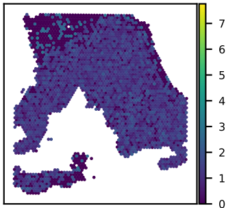
SNU18A DCTN4 expression Moran's I = 0.13
