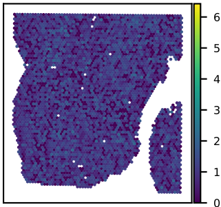
SNU25B CTNNBIP1 expression Moran's I = 0.02
