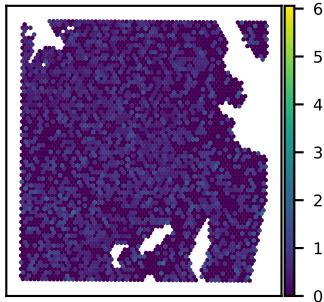
SNU51A FAM76B expression Moran's I = 0.01
