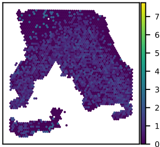
SNU18A PODXL expression Moran's I = 0.14
