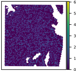
SNU51A WDFY2 expression Moran's I = 0.01
