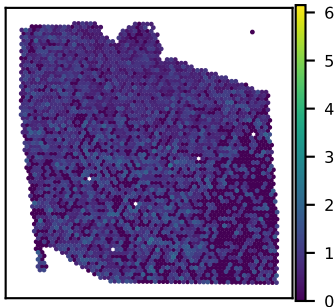
SNU27A PPP2R5A expression Moran's I = 0.05
