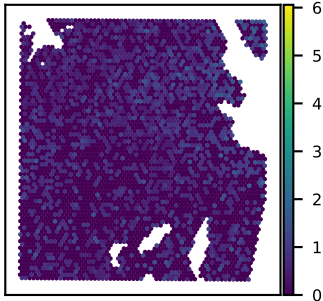
SNU51A MADD expression Moran's I = 0.06
