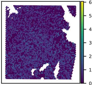
SNU51A BGLAP expression Moran's I = 0.05
