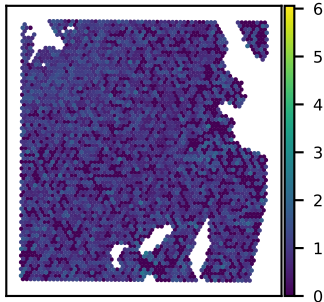
SNU51A C8orf33 expression Moran's I = 0.03
