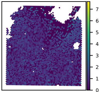
SNU21B TRIM56 expression Moran's I = 0.10
