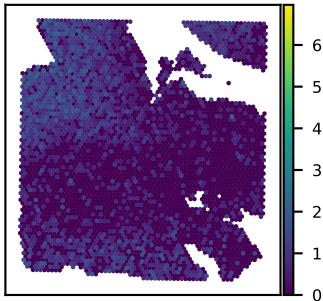
SNU24B KCNQ5 expression Moran's I = 0.40
