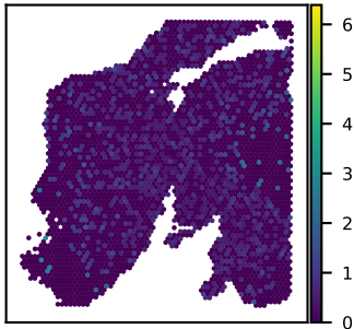
SNU24A SMYD4 expression Moran's I = 0.01
