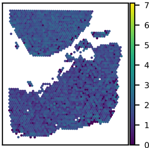
SNU25A SPTBN1 expression Moran's I = 0.07
