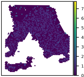
SNU18A RPUSD1 expression Moran's I = 0.07
