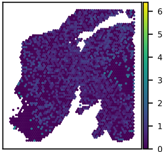
SNU24A MAP3K5 expression Moran's I = 0.06
