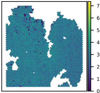
SNU27B HNRNPDL expression Moran's I = 0.14
