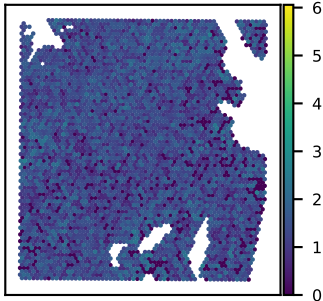
SNU51A C4orf3 expression Moran's I = 0.05
