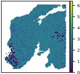
SNU24A SCARB2 expression Moran's I = 0.14
