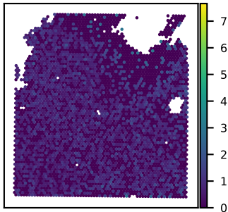
SNU21B ELMSAN1 expression Moran's I = 0.04
