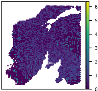
SNU24A GPATCH4 expression Moran's I = 0.05
