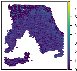
SNU18A GRAMD1A expression Moran's I = 0.17
