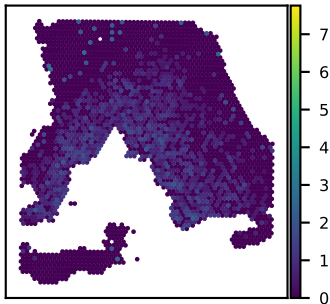
SNU18A PRIMA1 expression Moran's I = 0.32
