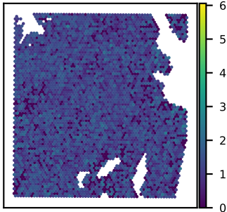
SNU51A PSMC4 expression Moran's I = 0.03
