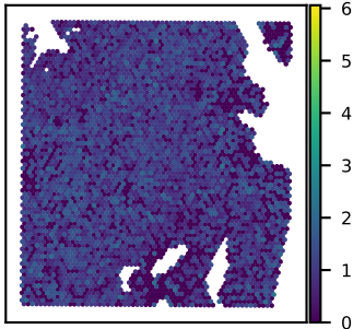
SNU51A RFTN2 expression Moran's I = 0.09
