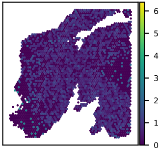
SNU24A CNOT6 expression Moran's I = 0.05
