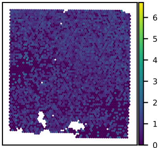
SNU43A GRAMD1A expression Moran's I = 0.10
