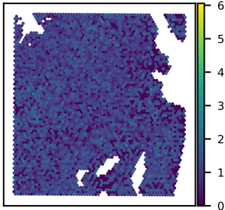
SNU51A CTNND1 expression Moran's I = 0.03
