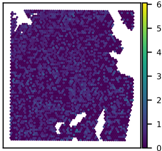
SNU51A SIRT7 expression Moran's I = 0.02
