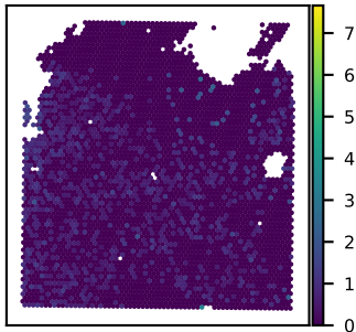
SNU21B SLC35F1 expression Moran's I = 0.13
