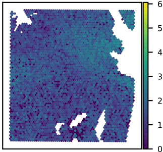
SNU51A SLC22A17 expression Moran's I = 0.25
