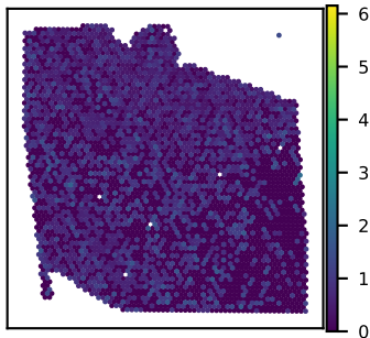
SNU27A CCDC159 expression Moran's I = 0.04
