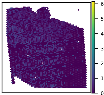
SNU27A SSUH2 expression Moran's I = 0.10
