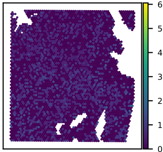
SNU51A RFC5 expression Moran's I = 0.02
