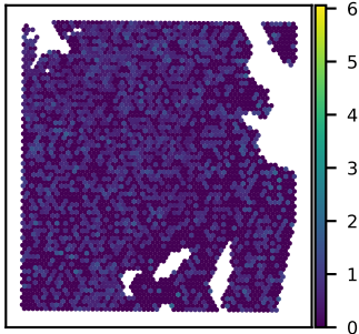
SNU51A CALCRL expression Moran's I = 0.03
