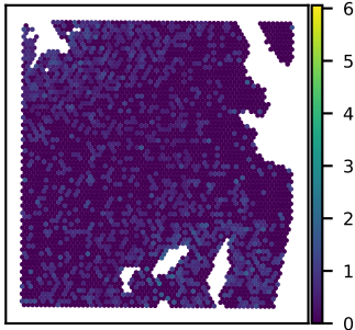
SNU51A RGS16 expression Moran's I = 0.10
