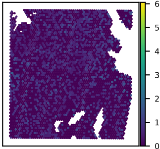
SNU51A TMEM192 expression Moran's I = 0.03
