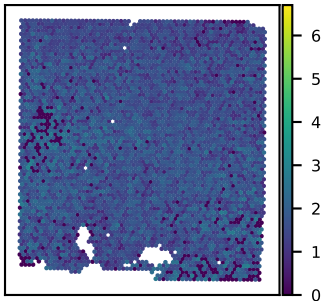
SNU43A C19orf53 expression Moran's I = 0.06
