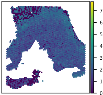
SNU18A TAPBP expression Moran's I = 0.32
