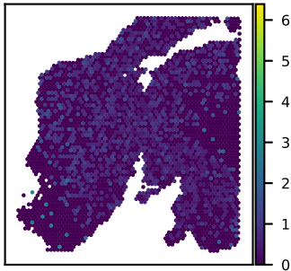
SNU24A PRAM1 expression Moran's I = 0.04
