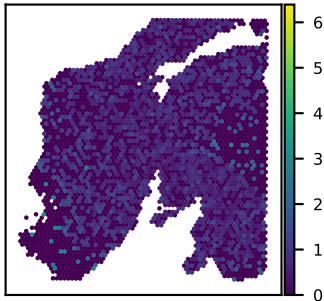
SNU24A ANAPC1 expression Moran's I = 0.03
