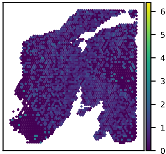
SNU24A CNOT6L expression Moran's I = 0.08
