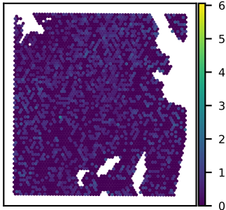
SNU51A FAXDC2 expression Moran's I = 0.04
