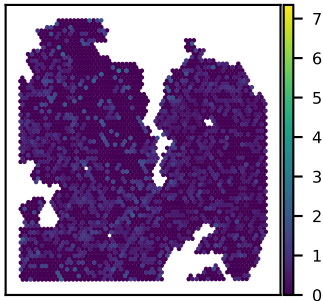
SNU27B LRRC37A2 expression Moran's I = 0.03
