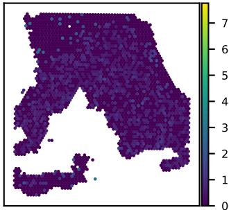
SNU18A TRIM35 expression Moran's I = 0.04
