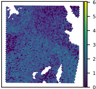
SNU51A HIST1H2AE expression Moran's I = 0.27
