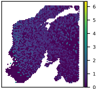
SNU24A C21orf91 expression Moran's I = 0.11
