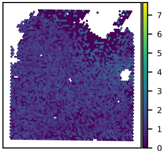
SNU21B CREM expression Moran's I = 0.14
