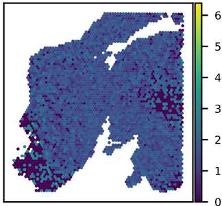
SNU24A POLR2I expression Moran's I = 0.09
