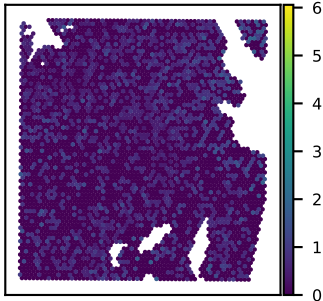
SNU51A PITRM1 expression Moran's I = 0.02
